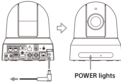
To the AC adapter (supplied)
